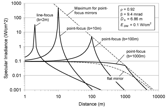
Fig. 5 Specular irradiance at the cornea as a function of distance from point-focus and line-focus mirrors with different focal lengths, b , for a solar irradiance of 0.1 W/cm 2
